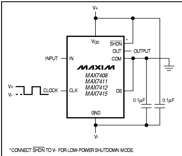
Figure 4. Dual-Supply Operation
