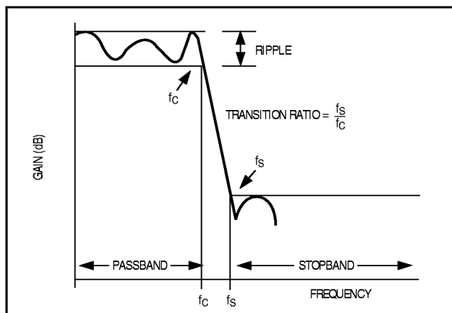
Figure 2. Elliptic Filter Response
