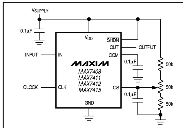
Figure 3. Offset Adjustment Circuit
